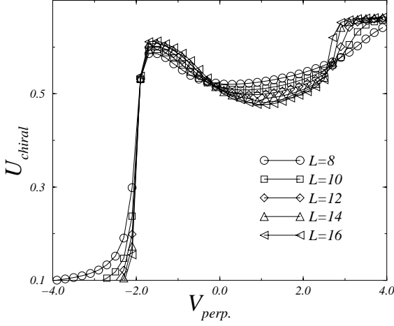
Fig. 1. Binder parameter for the chiral order (7) is plotted for t_{\parallel} = 1 , t_{\perp} = 0.5 , V_{\parallel} = 0.6 and various V_{\perp} . The symbols ( \circ ), ( \square ), ( \diamond ), ( \triangle ) and ( \triangleleft ) denote the data for the system sizes L = 8, 10, 12, 14 and 16 , respectively. We see that the chiral order develops in the repulsive interchain coupling -1.8 \lesssim V_{\perp} \lesssim 0 .
