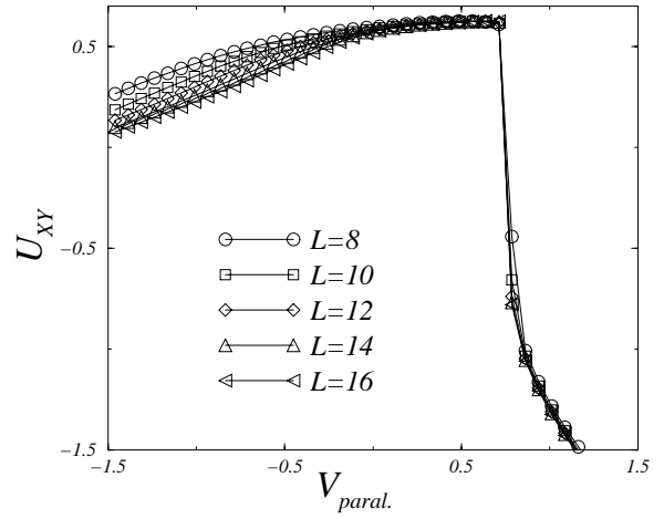
Fig. 4. Binder parameter for the XY order (9) is plotted for t_{\parallel} = 1 , t_{\perp} = 0.5 , V_{\perp} = -1 and various V_{\parallel} . The symbols ( \circ ), ( \square ), ( \diamond ), ( \triangle ) and ( \triangleleft ) denote the data for the system sizes L = 8, 10, 12, 14 and 16 , respectively. The XY order becomes disordered eventually in the repulsive intrachain coupling V_{\parallel} \gtrsim 0 and driven to spin-liquid phase.
