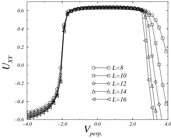
Fig. 3. Binder parameter for the XY order (9) is plotted for t_{\parallel} = 1 , t_{\perp} = 0.5 , V_{\parallel} = 0.6 and various V_{\perp} . The symbols ( \circ ), ( \square ), ( \diamond ), ( \triangle ) and ( \triangleleft ) denote the data for the system sizes L = 8, 10, 12, 14 and 16 , respectively. The XY order appears to be critical in the region -1.8 \lesssim V_{\perp} \lesssim 2.5 . In the region, the fixed point value of the Binder parameter seems to be unchanged. Hence, we see that the XY order is not influenced by the change of V_{\perp} .
