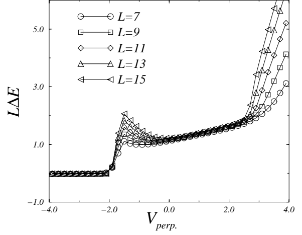
Fig. 2. Scaled kink energy (8) is plotted for the same parameter range as that of Figure 1. The symbols ( \circ ), ( \square ), ( \diamond ), ( \triangle ) and ( \triangleleft ) denote the data for the system sizes L = 7, 9, 11, 13 and 15 , respectively. In the region -1.8 \lesssim V_{\perp} \lesssim 0 , where the chiral phase is realized (see Fig. 1), the scaled kink energy grows actually. On the contrary, in the attractive region V_{\perp} \gtrsim 0 , the scaled kink energy stays scale-invariant. This indicates that a critical phase, probably of the XY mode, is realized; see Figure 3.
